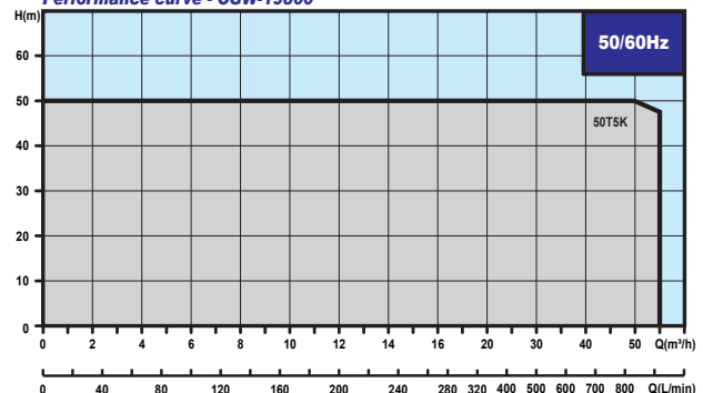
Performance curve - CGW-19800
