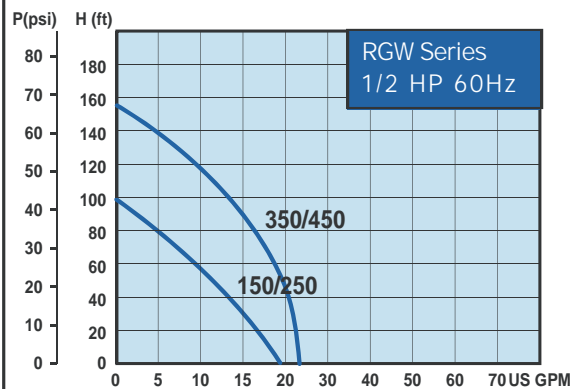
Hydraulic Performance curve:
